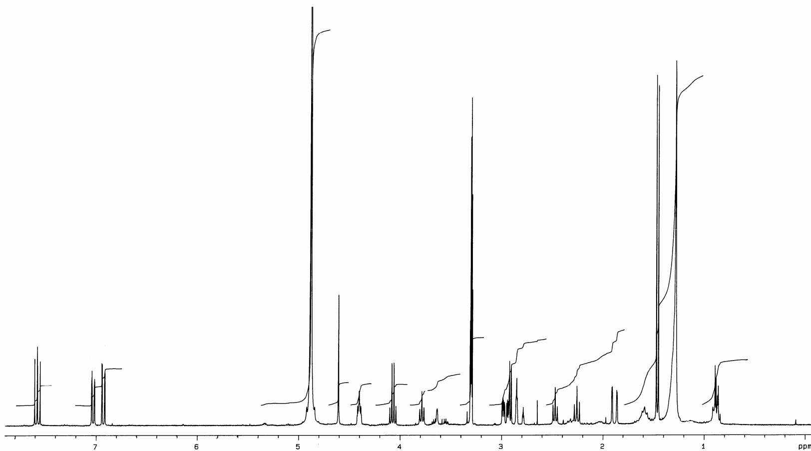
Figure S6. 1 H NMR spectrum of [(1 S *,3 R *,4 aS *,5 R *,10 aR *)-4 a ,5,9,10 a -tetrahydroxy-1-methyl-10-oxo-3,4,4 a ,5,10,10 a -hexahydro-1 H -benzo[ g ]isochromen-3-yl]-acetic acid-4 a -lactone ( 3b ) in [D 4 ]MeOD.
