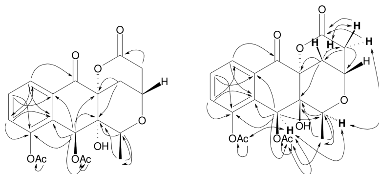
Fig. 4. HMBC (→) and selected NOESY (⇌) correlations (distance > 3 bonds) of oxidation products 4a (left) and 4b (right).
