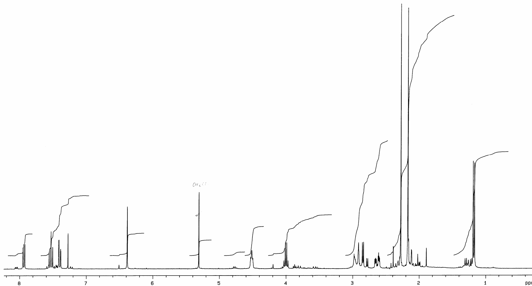
Figure S8. ^1\text{H} NMR spectrum of [(1S^*, 3R^*, 4aR^*, 10S^*, 10aR^*)\text{-}9,10\text{-diacetoxy-}4\text{a},10\text{-dihydroxy-}1\text{-methyl-}5\text{-oxo-}3,4,4\text{a},5,10,10\text{-hexahydro-}1\text{H-benzo[g]isochromen-}3\text{-yl)]\text{-acetic acid-}4\text{a-lactone} ( 4b ) in \text{CDCl}_3 .
